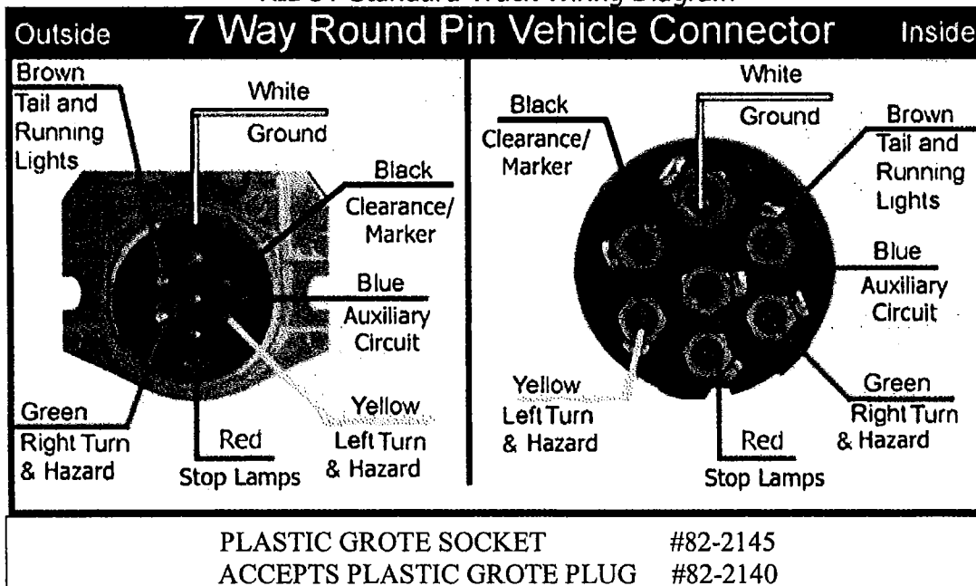
RIDOT Standard Truck Wiring Diagram
