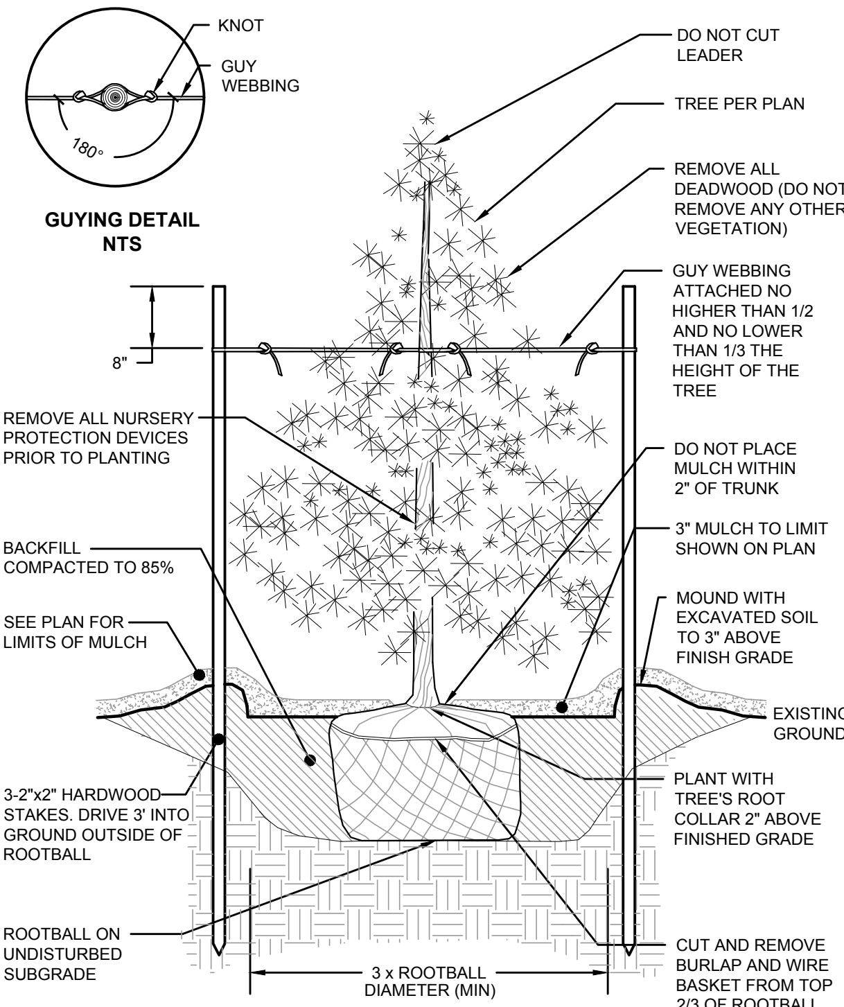
EVERGREEN TREE STAKING & PLANTING NOT TO SCALE
