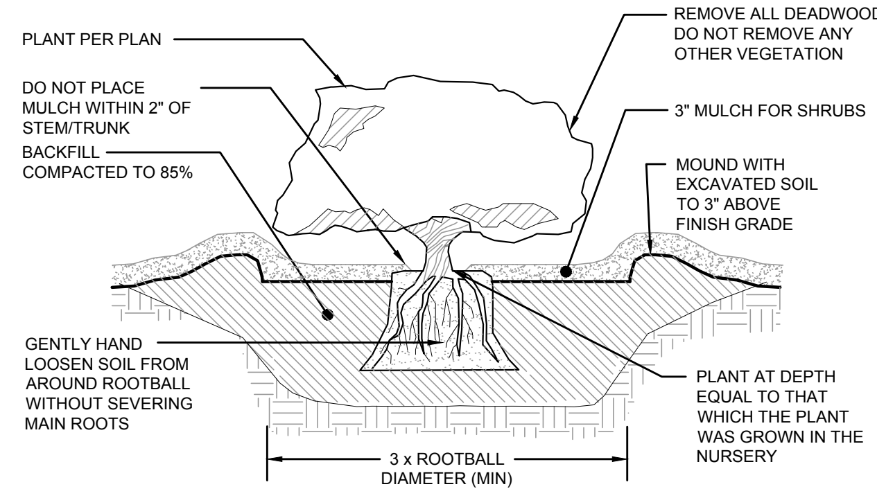
CONTAINER GROWN SHRUB PLANTING NOT TO SCALE
