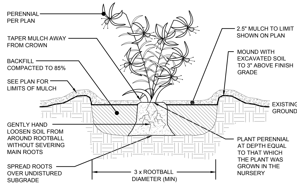
PERENNIALS & GRASSES PLANTING NOT TO SCALE
