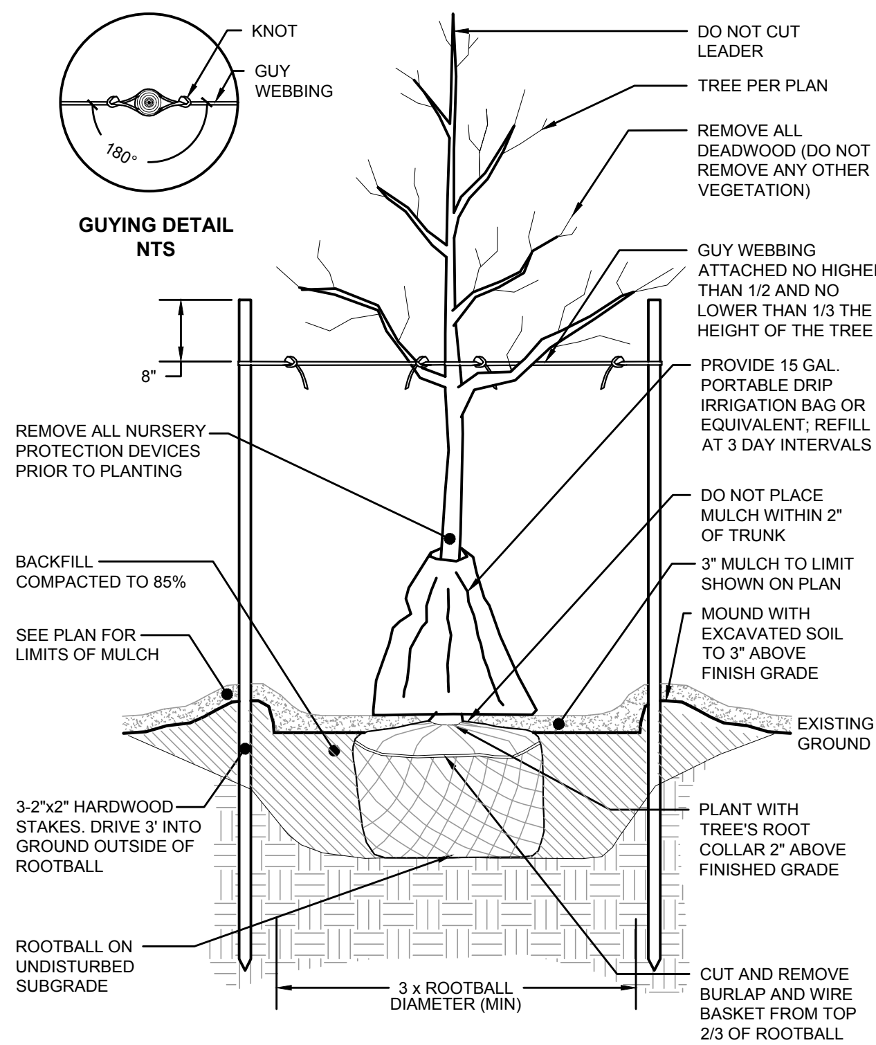
DECIDUOUS TREE STAKING & PLANTING NOT TO SCALE
