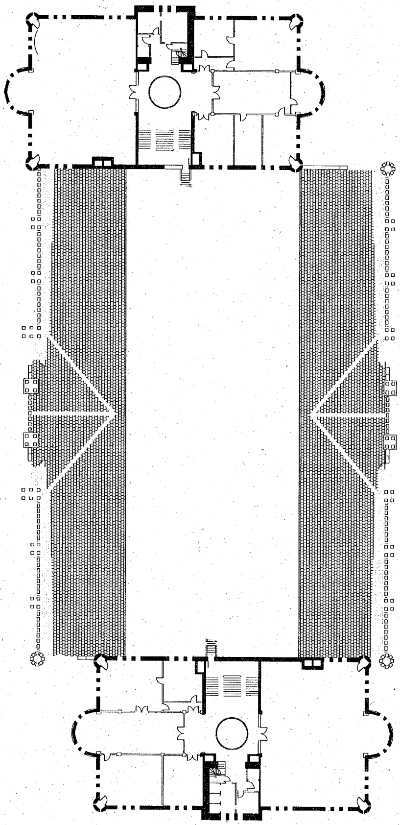
Fourth Floor
