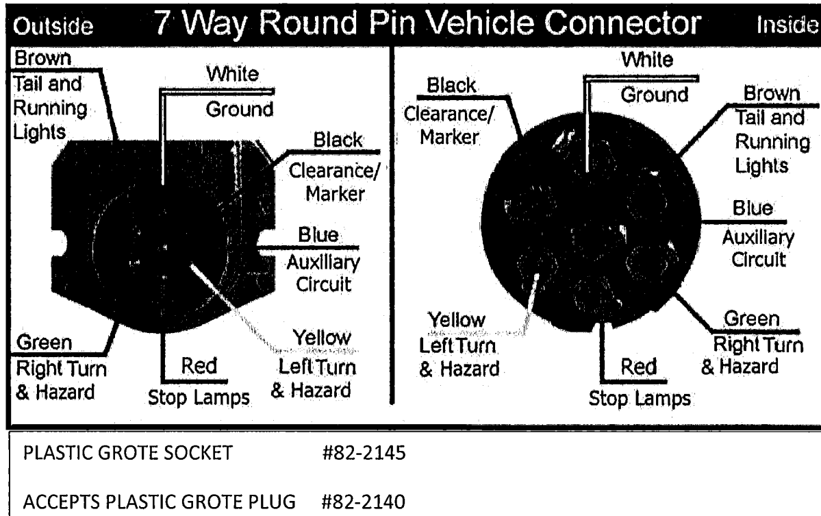
RIDOT Standard Truck Wiring Diagram
