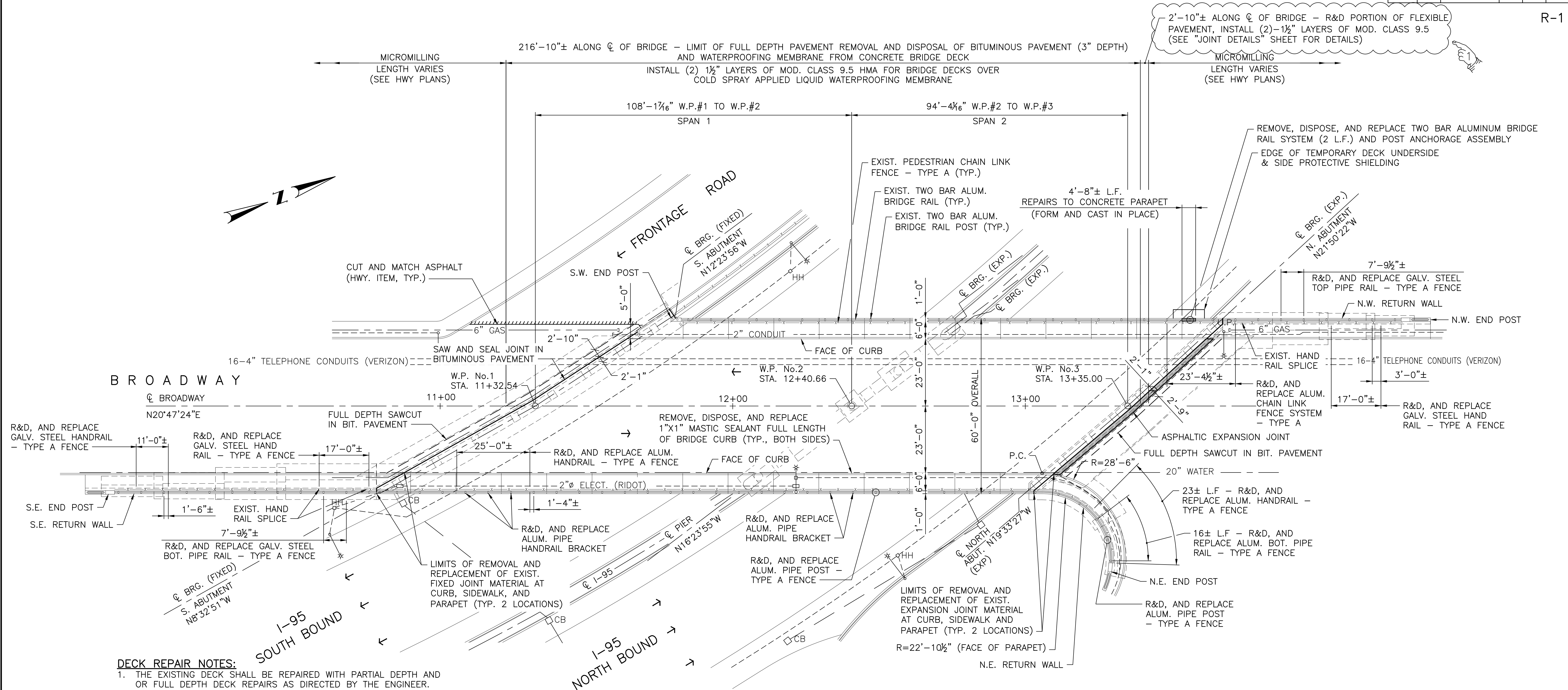
BRIDGE GENERAL PLAN SCALE 1"=16'-0"
